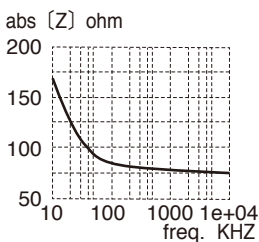
High frequency characteristics of Part No.2964 and #2965.
