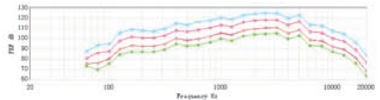
Frequency Response of VSS210 Measured at 5 cm from Outlet in the Anechoic Chamber
