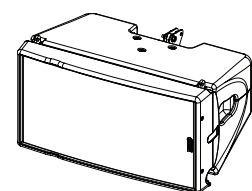
GEO M1012-I Line array element, 2 way passive, 1 x 10 inches, install, black, 12.5° vertical, 80° horizontal, 59 Hz - 20 KHz, 131 dB, 21 Kg (GEO M1012-IPW for white version)
