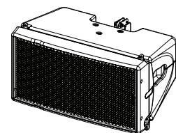
GEO M1025 Line array element, 2 way passive, 1 x 10 inches, touring, black, 25° vertical, 80° horizontal, 59 Hz - 20 KHz, 131 dB, 21 Kg (GEO M1025-PW for white version)
