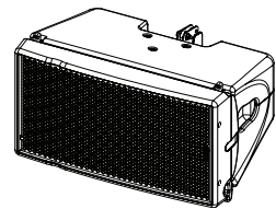
GEO M1012 Line array element, 2 way passive, 1 x 10 inches, touring, black, 12.5° vertical, 80° horizontal, 59 Hz - 20 KHz, 131 dB, 21 Kg (GEO M1012-PW for white version)
