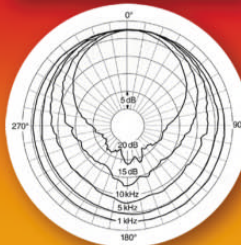
Omni Polar Pattern
