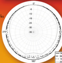
Omni Polar Pattern
