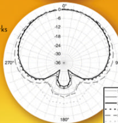
Cardioid Polar Pattern
